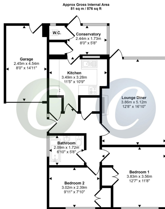
Floorplan
